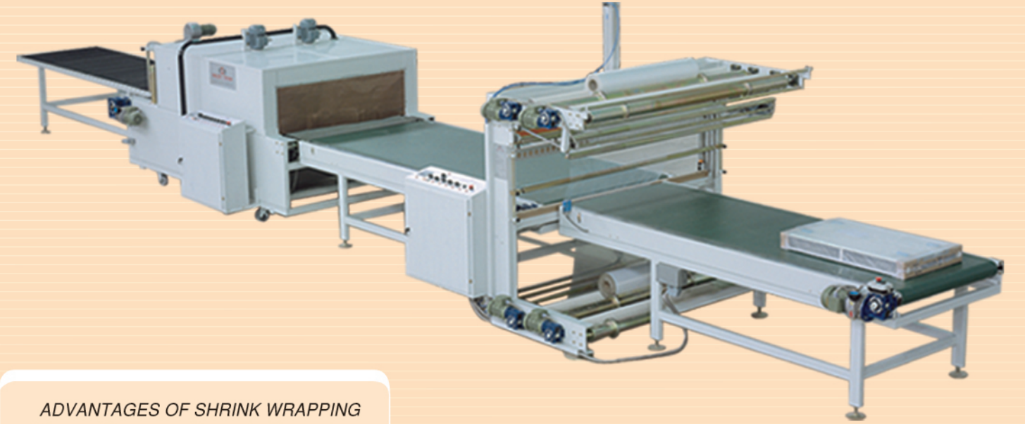
MT 1300 TAM OTOMATİK SHRINK MAKİNASI MT 1300 Full Automatic Shrink Wrapping Machine
